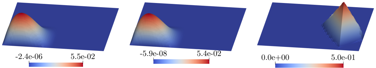
FIGURE 6. Deterministic solution: Control u_\tau^* (left), state \bar{y}_\tau^* (middle), multiplier \bar{\zeta}_\tau^* (right).
