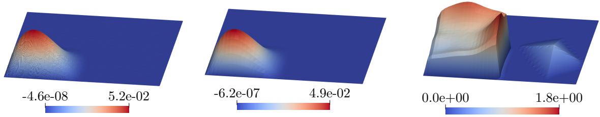
FIGURE 5. Lognormal noise: Control u_\tau^* (left), state \bar{y}_\tau^* (middle), multiplier \bar{\zeta}_\tau^* (right) for \beta = 0.95 .
