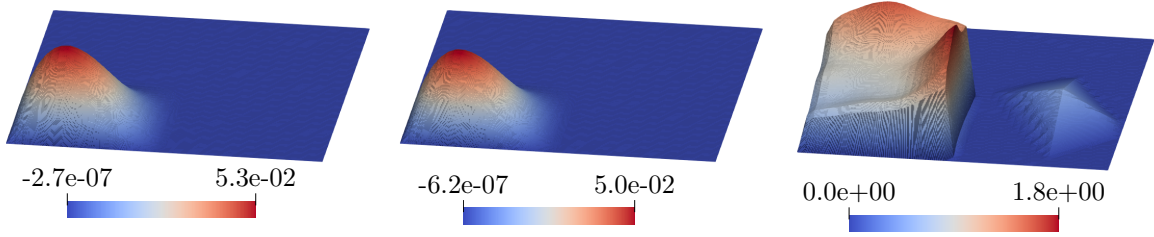
FIGURE 4. Lognormal noise: Control u_\tau^* (left), state \bar{y}_\tau^* (middle), multiplier \bar{\zeta}_\tau^* (right) for \beta = 0.0 .
