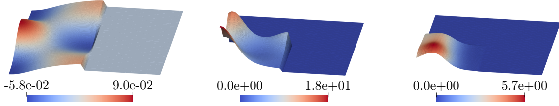
FIGURE 1. Example realisations of random field zero-mean b (left) and lognormal random fields b (middle, right).
