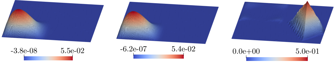
FIGURE 3. Mean-zero noise: Control u_\tau^* (left), state \bar{y}_\tau^* (middle), multiplier \bar{\zeta}_\tau^* (right) for \beta = 0.95 .
