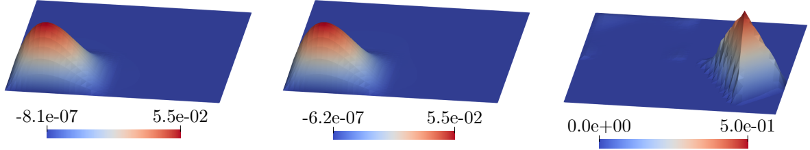
FIGURE 2. Mean-zero noise: Control u_\tau^* (left), state \bar{y}_\tau^* (middle), multiplier \bar{\zeta}_\tau^* (right) for \beta = 0.0 .
