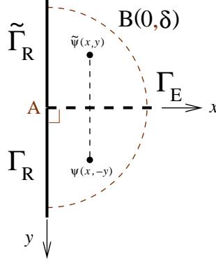
FIGURE 2. Fig. 2. Extension by parity in the proof of Theorem 4.1.
