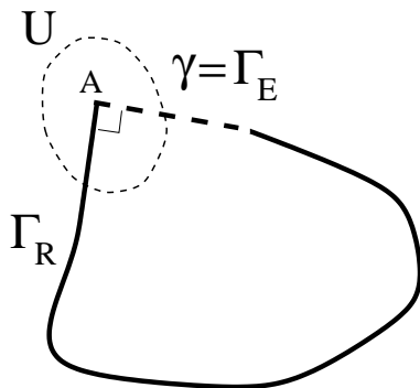
FIGURE 1. Shape of a domain satisfying conditions of Theorem 3.1.
