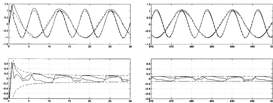
FIGURE 9. System (44) under funnel control (27) with funnel envelope (45). Upper: components of system output (solid lines) and reference signal (dashed lines). Lower: components of error (solid lines) and funnel boundary (dashed line).
