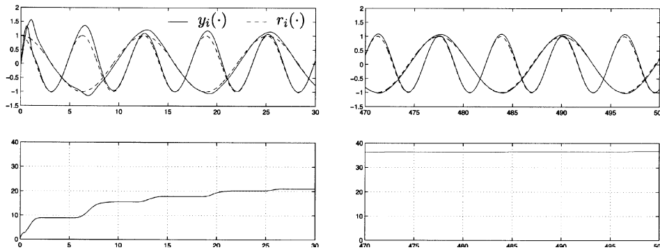
FIGURE 7. Adaptive \lambda -tracking control (47) of system (44). Upper: components of system output (solid lines) and reference signal (dashed lines). Lower: adaptive gain k(\cdot) .
