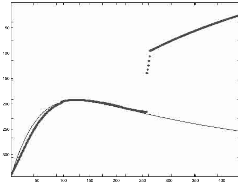
FIGURE 9. \mu(s) and \hat{\mu}_t(s) at time t = 0.051 .
