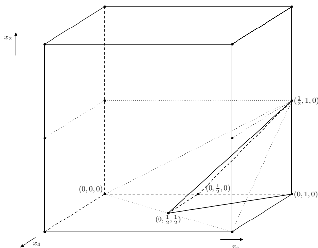
FIGURE 1. T = R_1 \cap \{x_1 = \frac{1}{2}\} \subset T_3 .
