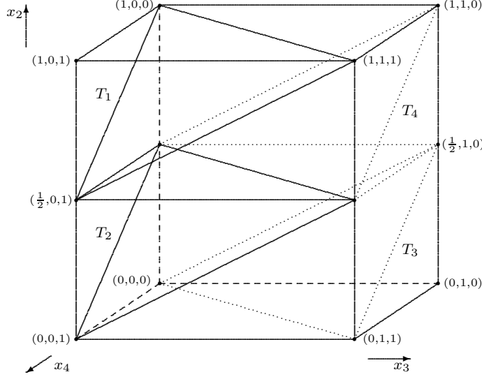
FIGURE 4. The tetrahedrons T_1, T_2, T_3, T_4 .
