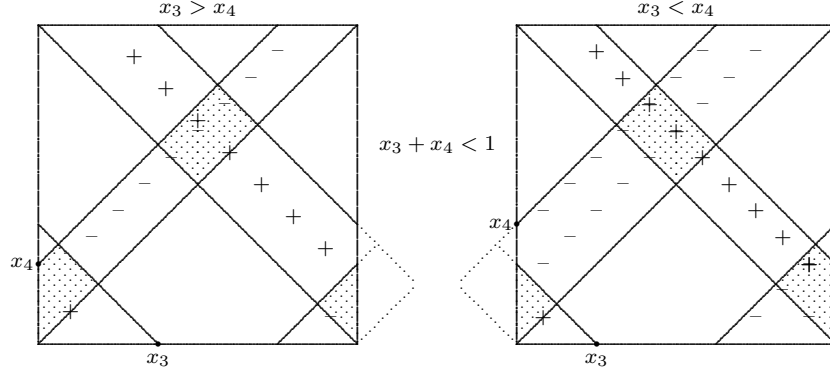
FIGURE 3. 2 \cdot \frac{x_3 x_4}{\sqrt{2} \sqrt{2}} = x_3 x_4 .
