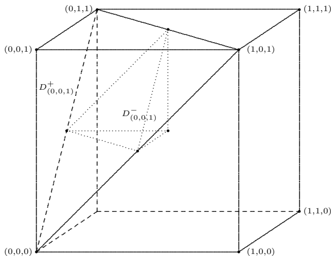
FIGURE 2. D_{(0,0,1)}^+ and D_{(0,0,1)}^- .
