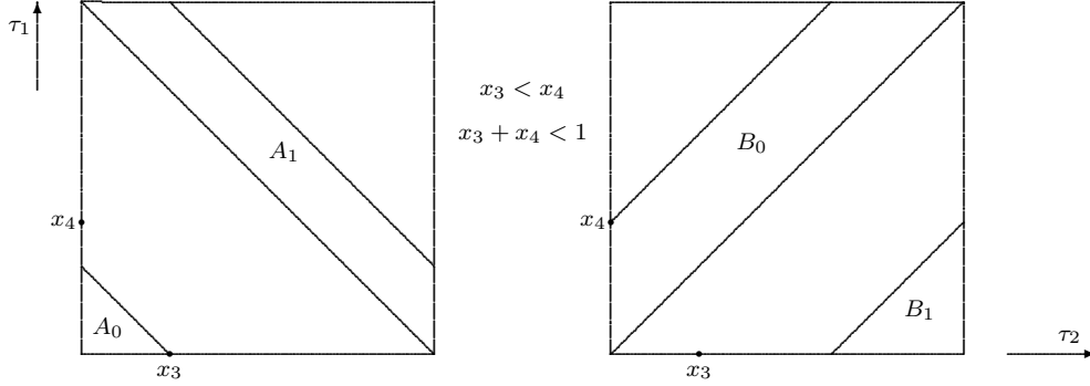
FIGURE 5. The sets A_0, A_1, B_0, B_1 .
