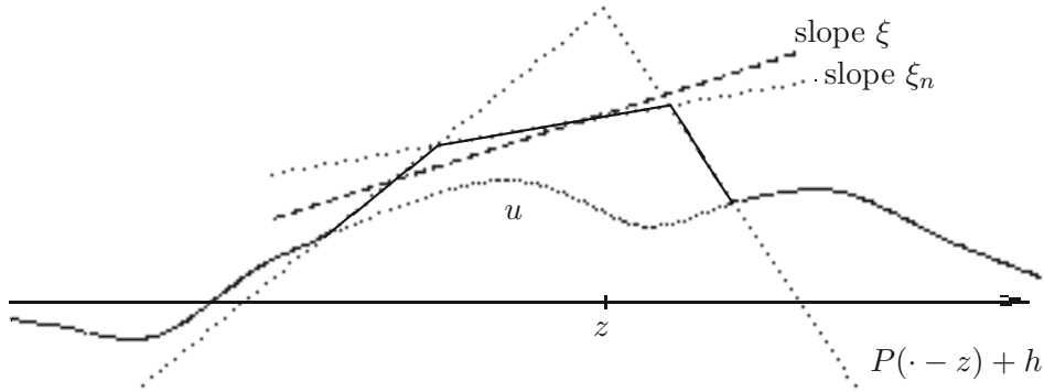
FIGURE 1. An example for w_n with \Omega = \mathbb{R} , in case \xi \in (\text{co } F)^\circ .
