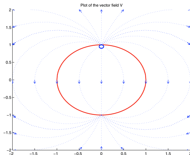
FIGURE 1. Phase portrait of the vector field V .
