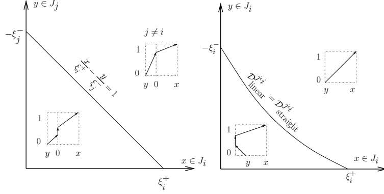
FIGURE 4. i, j \in I_N \setminus I_0 : trajectories do stay at the junction point if (y, x) \sim (0, 0) .
