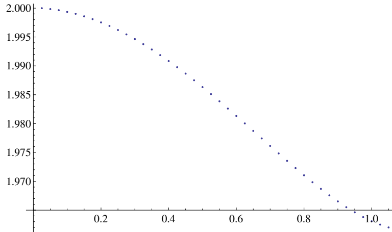
FIGURE 12. The map L \mapsto d_1 when the disk is transformed into an hexagon.
