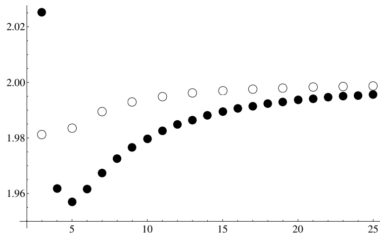
FIGURE 2. The maps n \mapsto d_1(\Omega_n) (regular polygons \bullet ) and n \mapsto d_1(R_n) (Reuleaux polygons \circ ).
