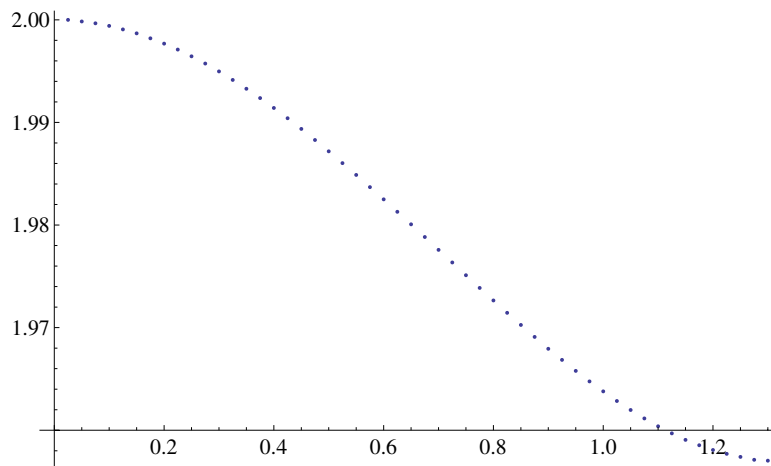
FIGURE 11. The map L \mapsto d_1(\Omega) when \Omega is deformed as in Figure 10.
