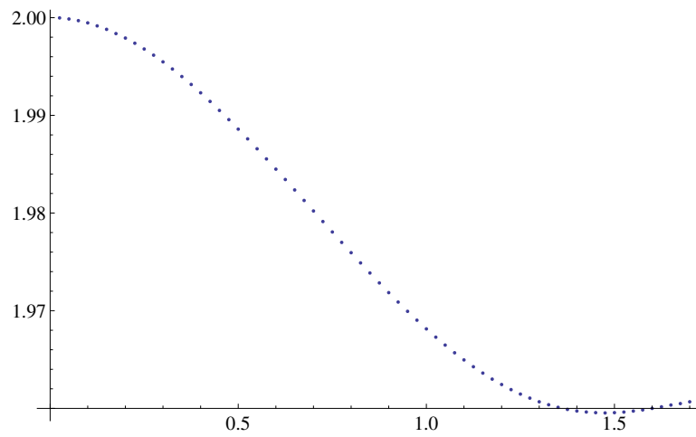
FIGURE 9. The map L \mapsto d_1 when the disk is transformed into a square.
