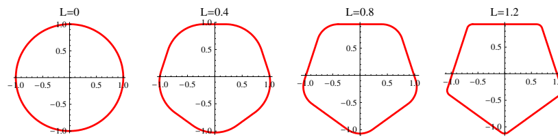
FIGURE 10. Deformation of the disk into a pentagon.
