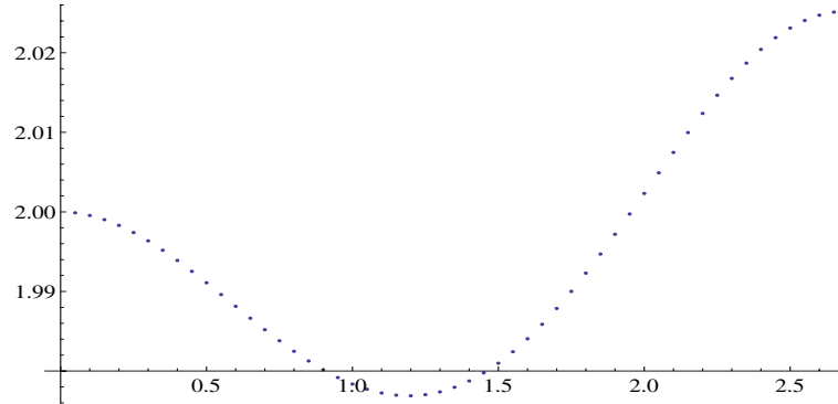
FIGURE 8. The map L \mapsto d_1(\Omega) when \Omega is deformed as in Figure 7.
