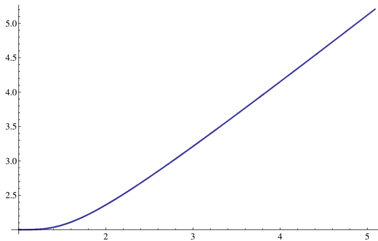
FIGURE 13. The map R \mapsto d_1 for ellipses from R = 1 (disk) to R \rightarrow \infty (segment).
