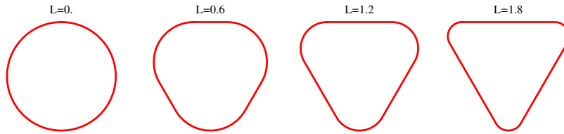
FIGURE 7. Deformation of the disk into a triangle.
