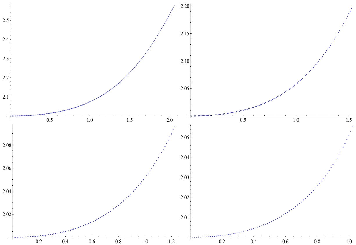
FIGURE 21. The maps L \mapsto d_1(\Omega) when \Omega is deformed from the disk to regular polygons \Omega_n^\sharp , n = 3, 4, 5, 6 .
