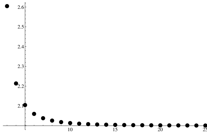
FIGURE 16. The map n \mapsto d_1(\Omega_n^\#) for regular n -polygons with perimeter equal to 2\pi .
