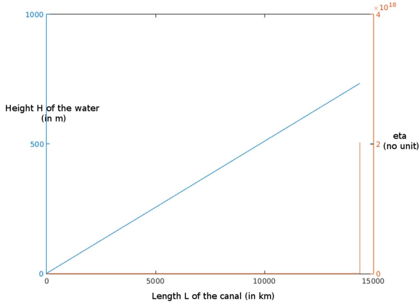
FIGURE 2. In the x -axis is represented the length of the water channel, in blue the height of the water in stationary state and in red the value of \eta , one can see the limit length L_{\max} at which \eta explodes.
