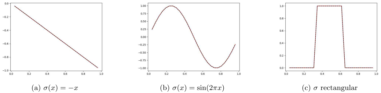
FIGURE 4. Different examples of reconstruction for h(t) = t + \sin(\pi t) .
