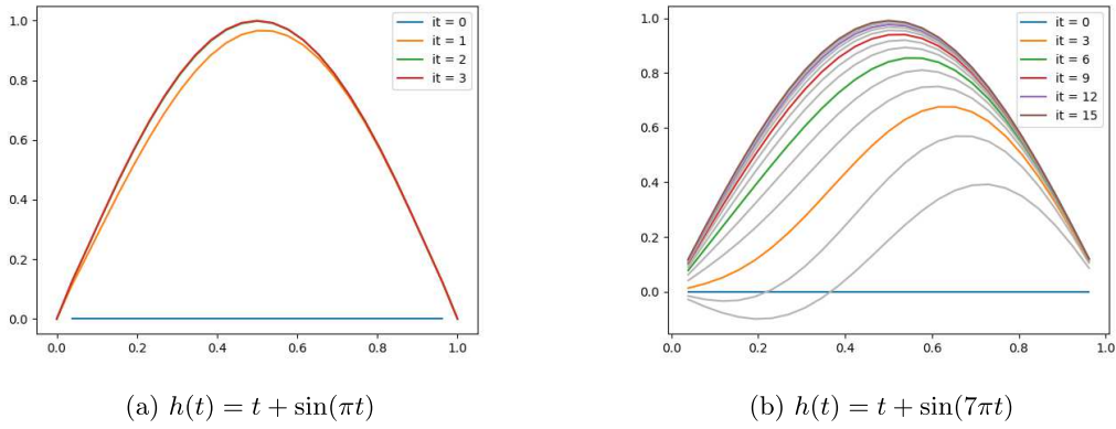
FIGURE 3. Reconstruction of \sigma(x) = \sin(\pi x) . Different choices for h and the corresponding convergence history.
