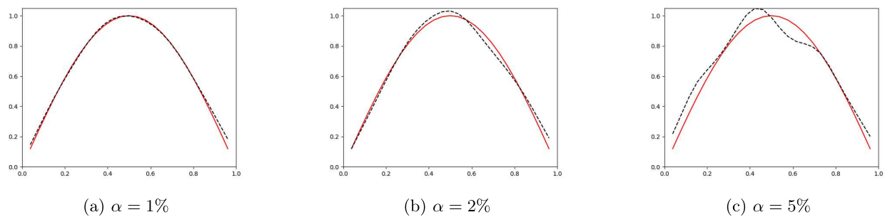
FIGURE 5. Reconstruction of the source \sigma(x) = \sin(\pi x) for h(t) = t + \sin(\pi t) in presence of noise in the data. The level of noise is denoted by \alpha .
