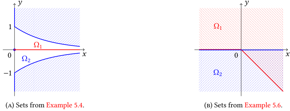
FIGURE 5.1. Visualization of the sets \Omega_1 and \Omega_2 from Examples 5.4 and 5.6.
