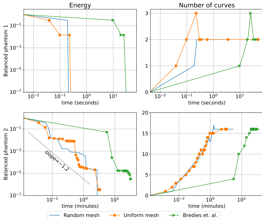
(B) Convergence of energy and sparsity of reconstructions. For each phantom, every energy is translated by the smallest energy found by any method.
